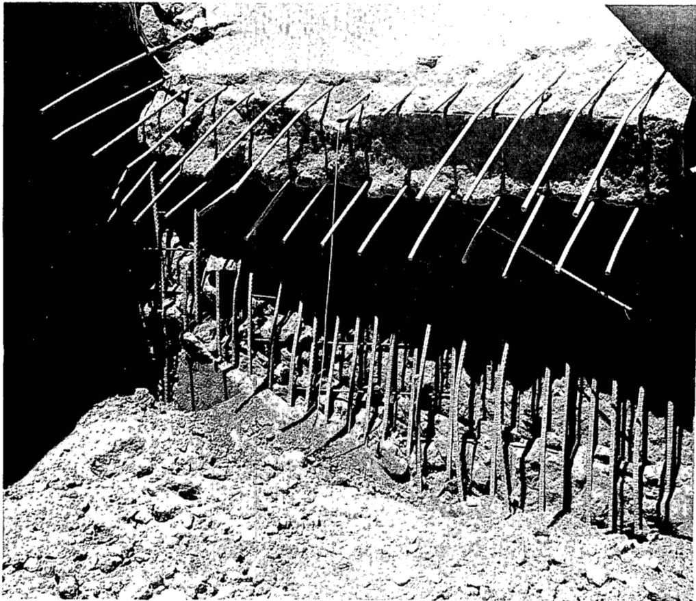
Fig. 2—Detail of failure showing fractured bars, postshot.
